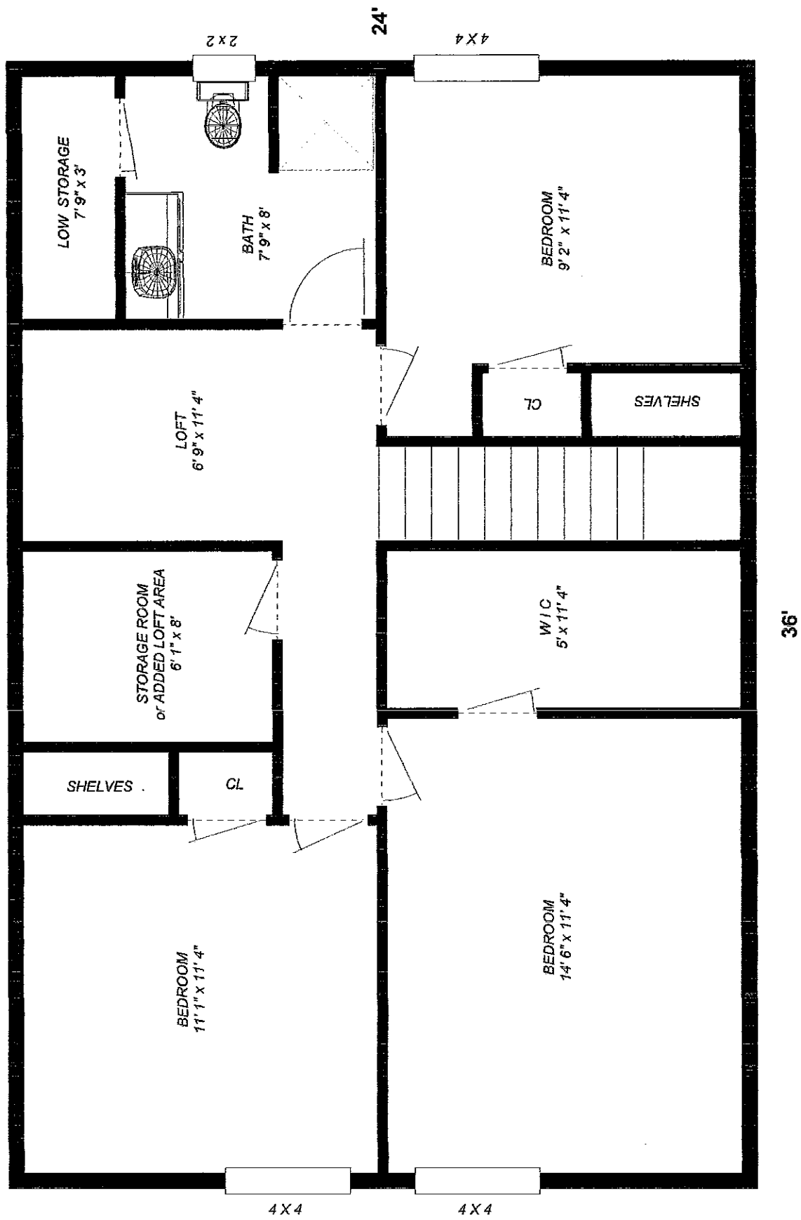
PLAN 7 24 X 28 1536 s.f. (2nd Floor)
